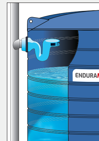
Siphon overflow
