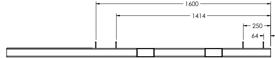
RIGHT VIEW
