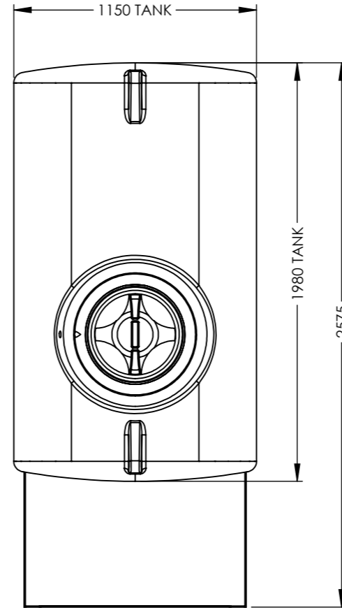
PLAN VIEW
